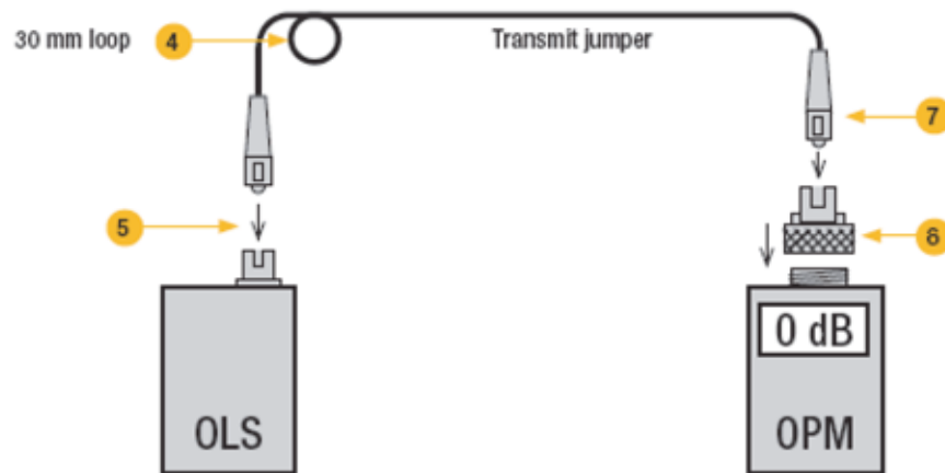
Fig. 4—Set Reference, Single-mode Link
