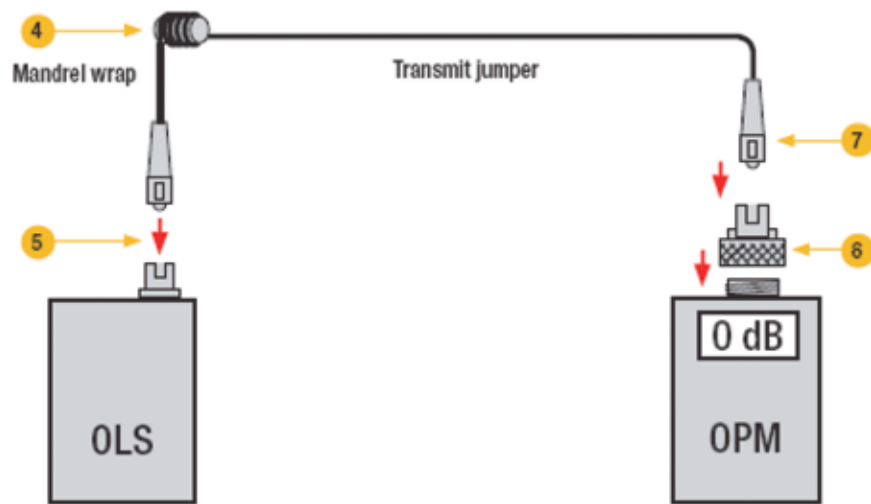
Fig. 1—Set Reference, Multimode Link
