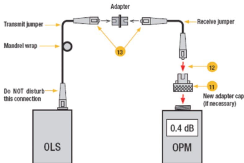
Fig. 2—Verify Test Jumpers, Multimode Link
